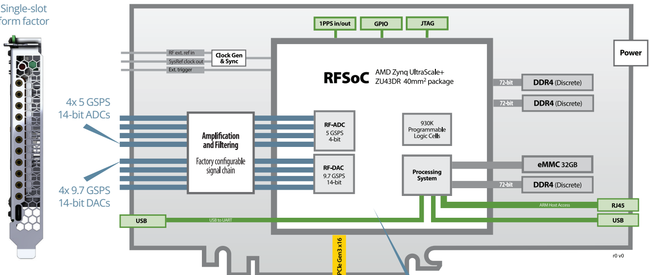
3rd generation RFSoc with dual ARM and FPGA
